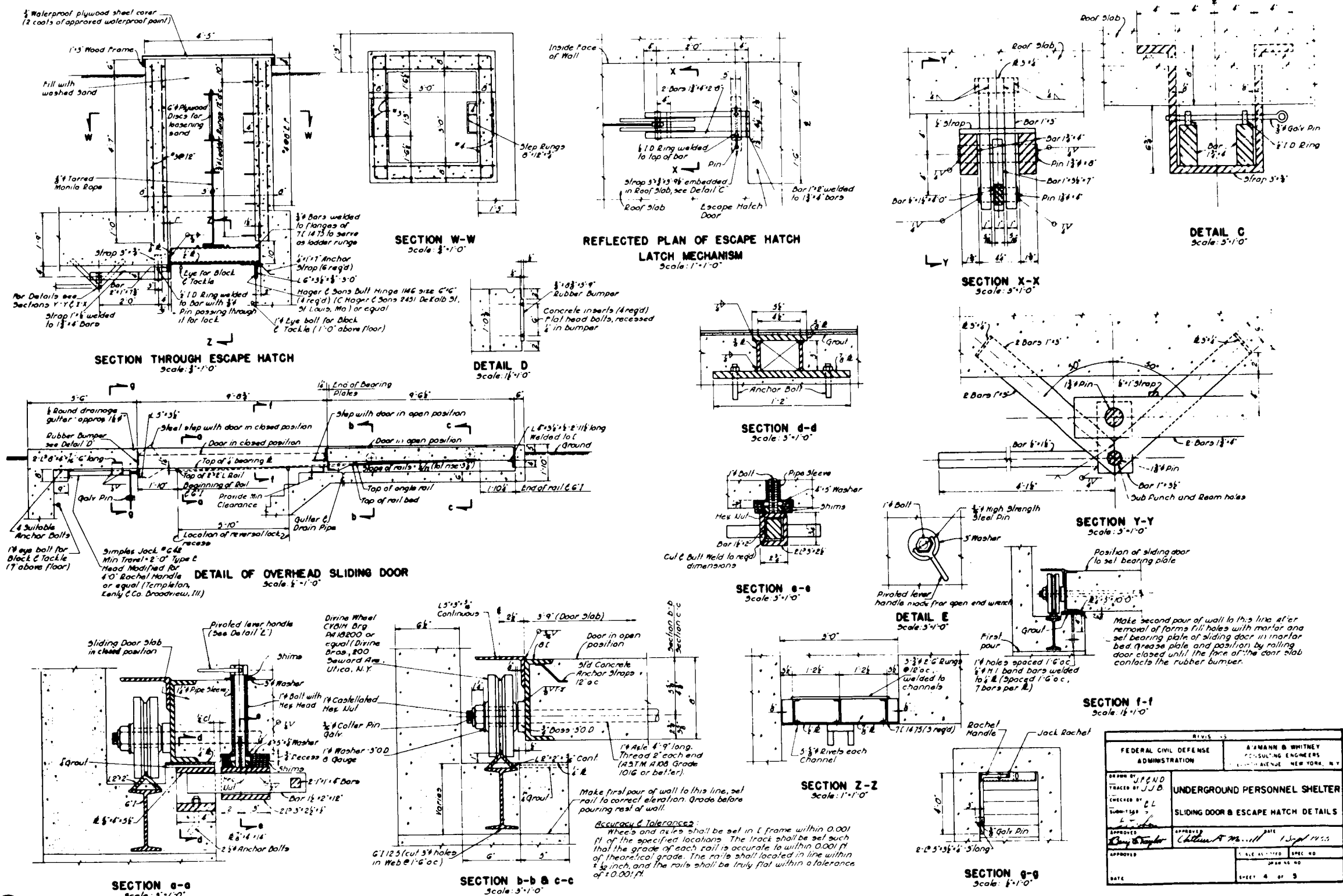
Fig. 18—Sliding-door and escape-hatch details, underground personnel shelter.
